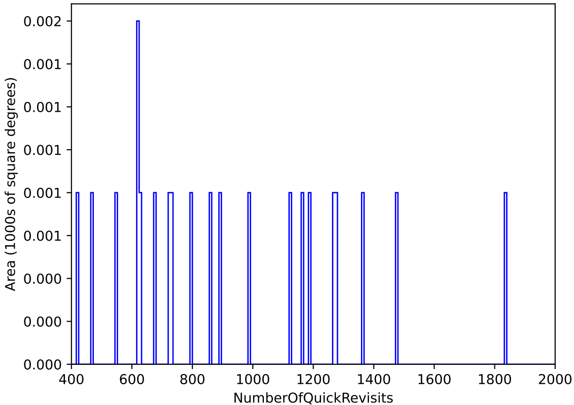
ddf_acor_sf10_lsf20_lsr10_v3.4_10yrs : NumberOfQuickRevisits
