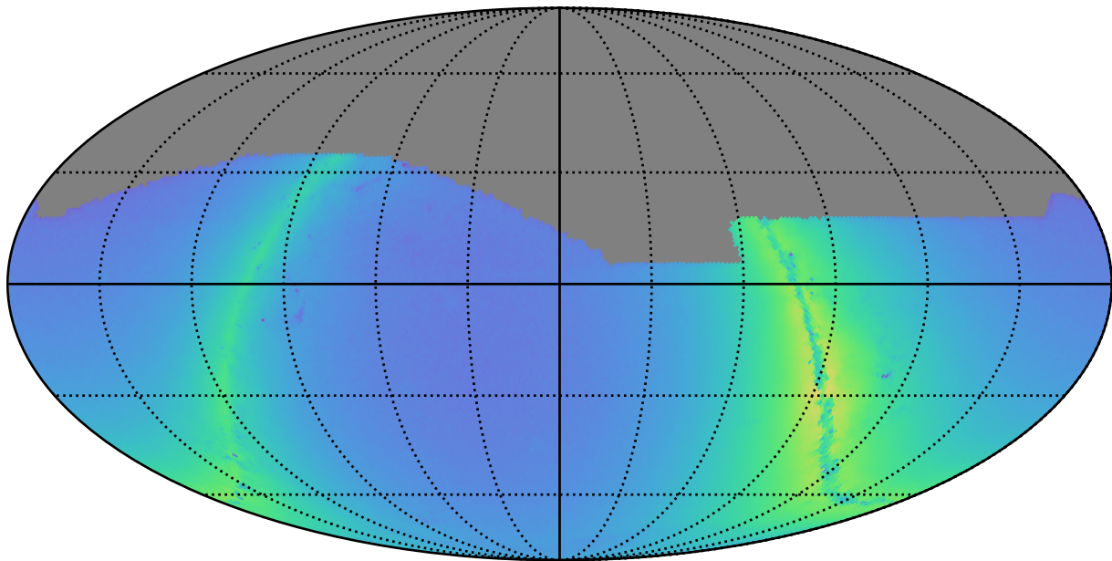
ddf_acor_sf10_lsf20_lsr10_v3.4_10yrs r: Nstars_no_crowding
