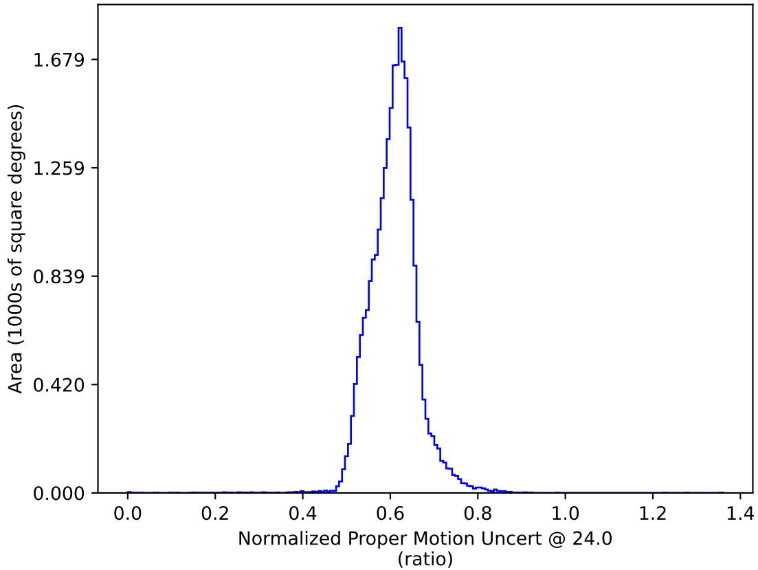
ddf_acor_sf10_lsf20_lsr10_v3.4_10yrs : Normalized Proper Motion Uncert @ 24.0
