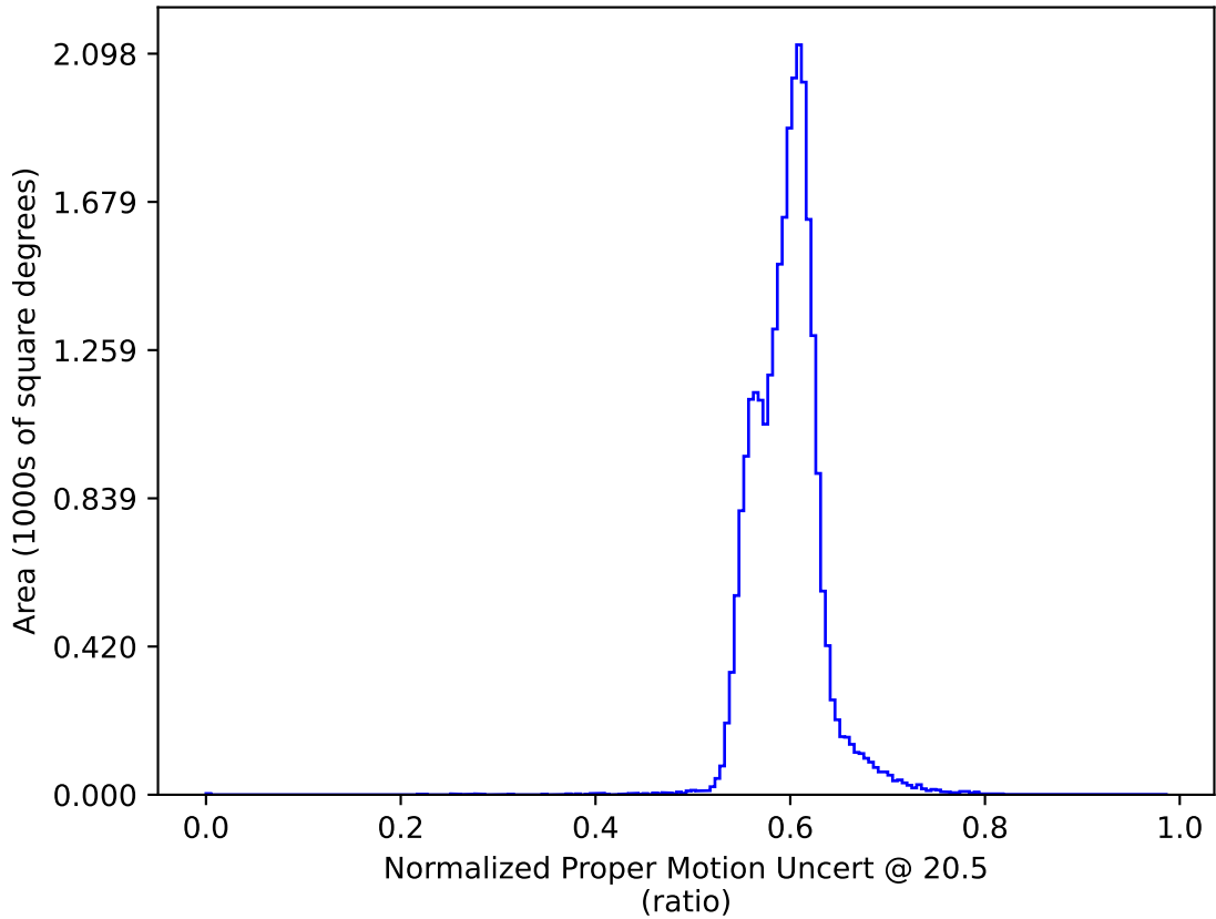
ddf_acor_sf10_lsf20_lsr10_v3.4_10yrs : Normalized Proper Motion Uncert @ 20.5
