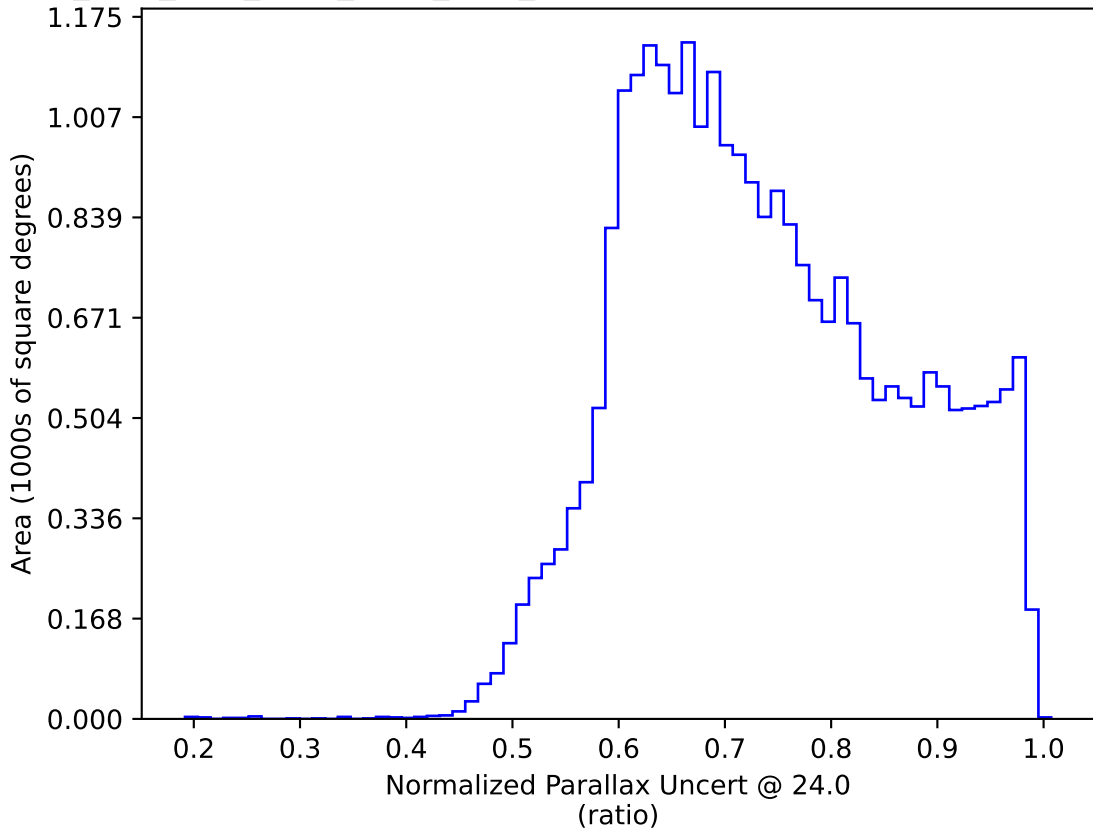
ddf_acor_sf10_lsf20_lsr10_v3.4_10yrs : Normalized Parallax Uncert @ 24.0
