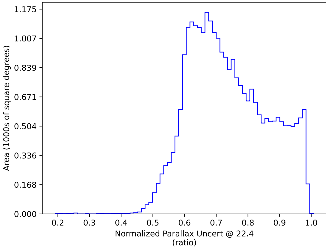
ddf_acor_sf10_lsf20_lsr10_v3.4_10yrs : Normalized Parallax Uncert @ 22.4
