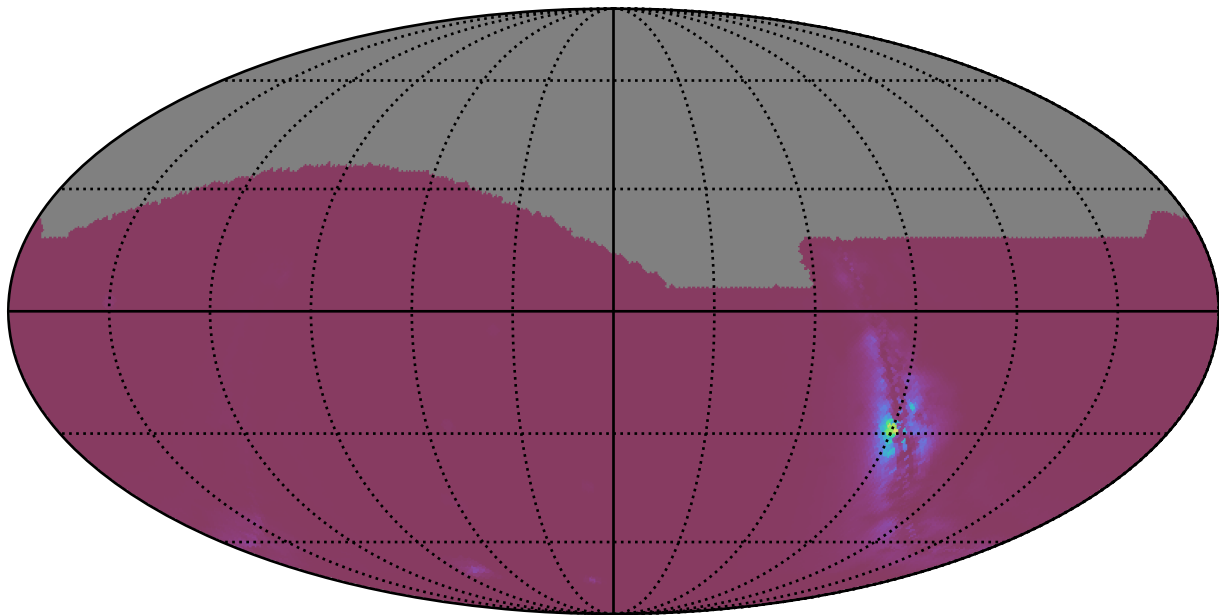
ddf_acor_sf10_lsf20_lsr10_v3.4_10yrs : NlcPoints
