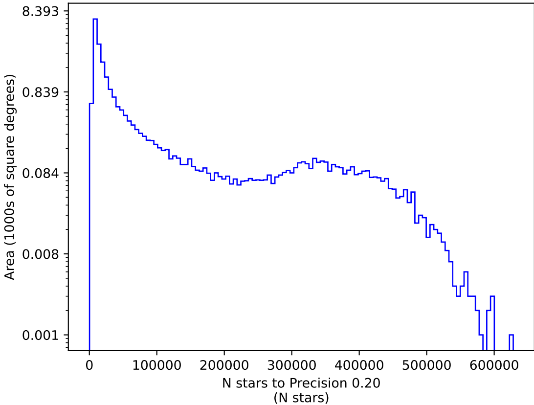
ddf_acor_sf10_lsf20_lsr10_v3.4_10yrs y: N stars to Precision 0.20
