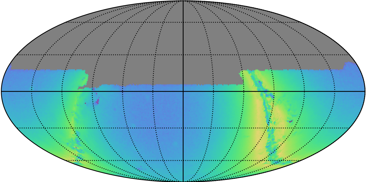
ddf_acor_sf10_lsf20_lsr10_v3.4_10yrs u: N stars to Precision 0.20
