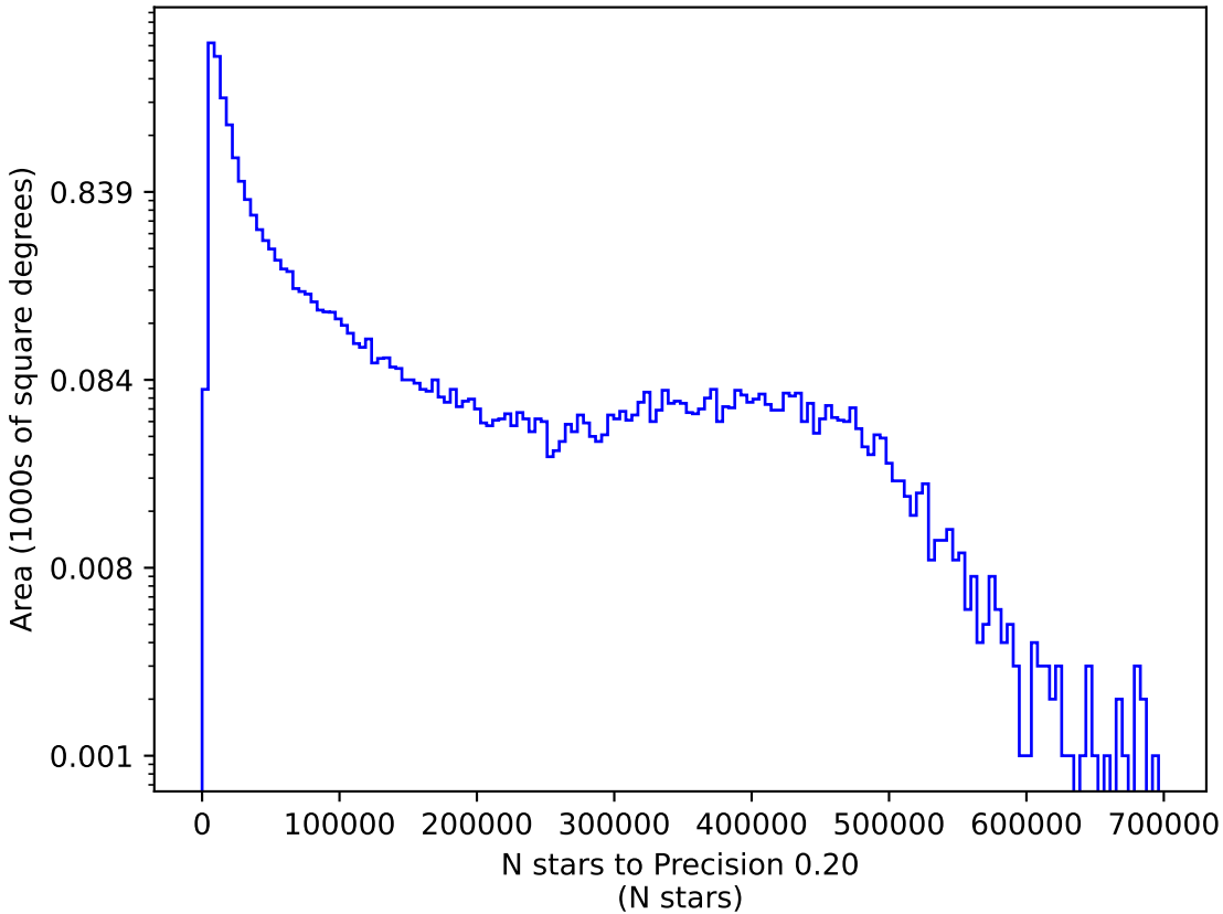
ddf_acor_sf10_lsf20_lsr10_v3.4_10yrs r: N stars to Precision 0.20
