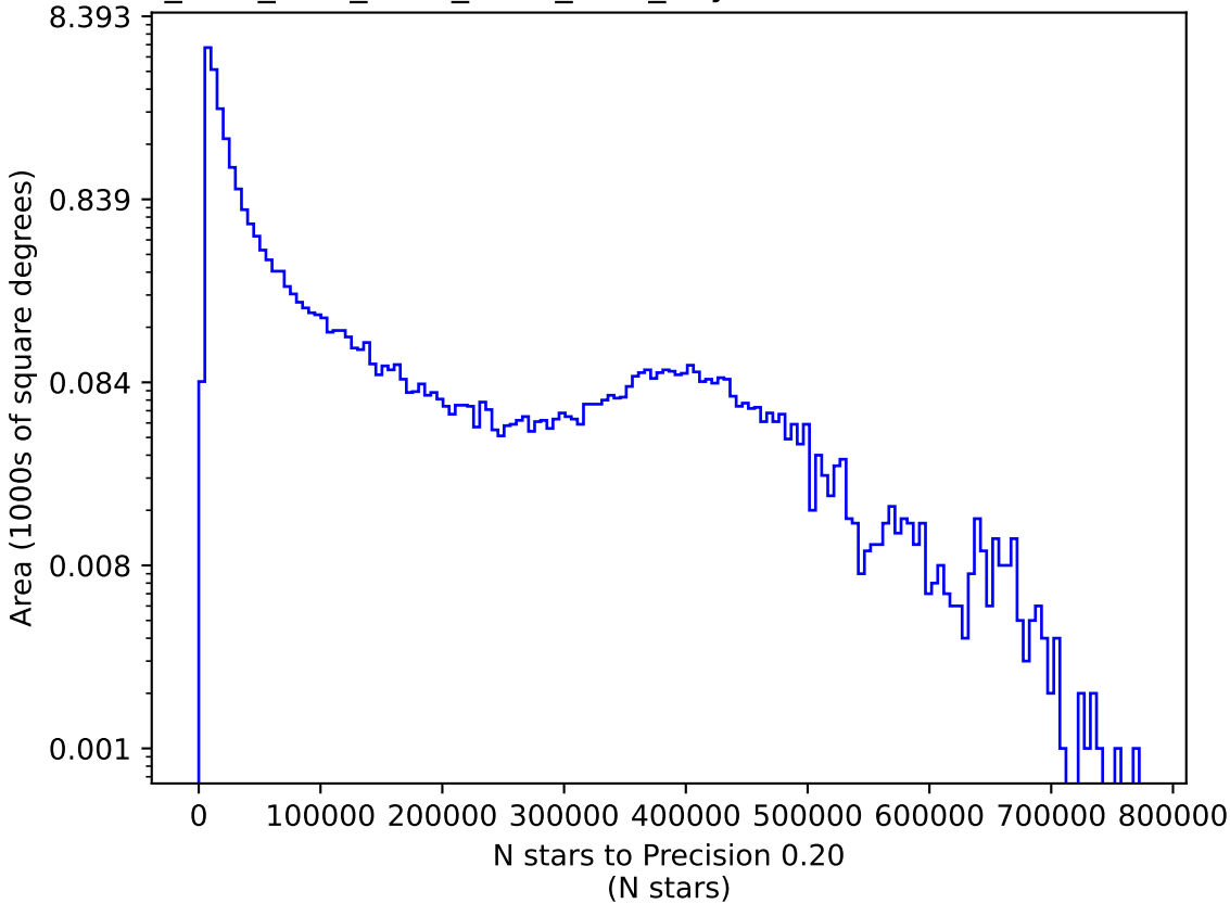
ddf_acor_sf10_lsf20_lsr10_v3.4_10yrs i: N stars to Precision 0.20
