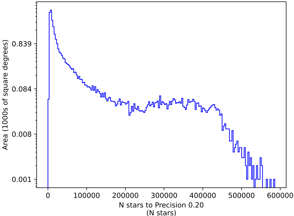
ddf_acor_sf10_lsf20_lsr10_v3.4_10yrs g: N stars to Precision 0.20
