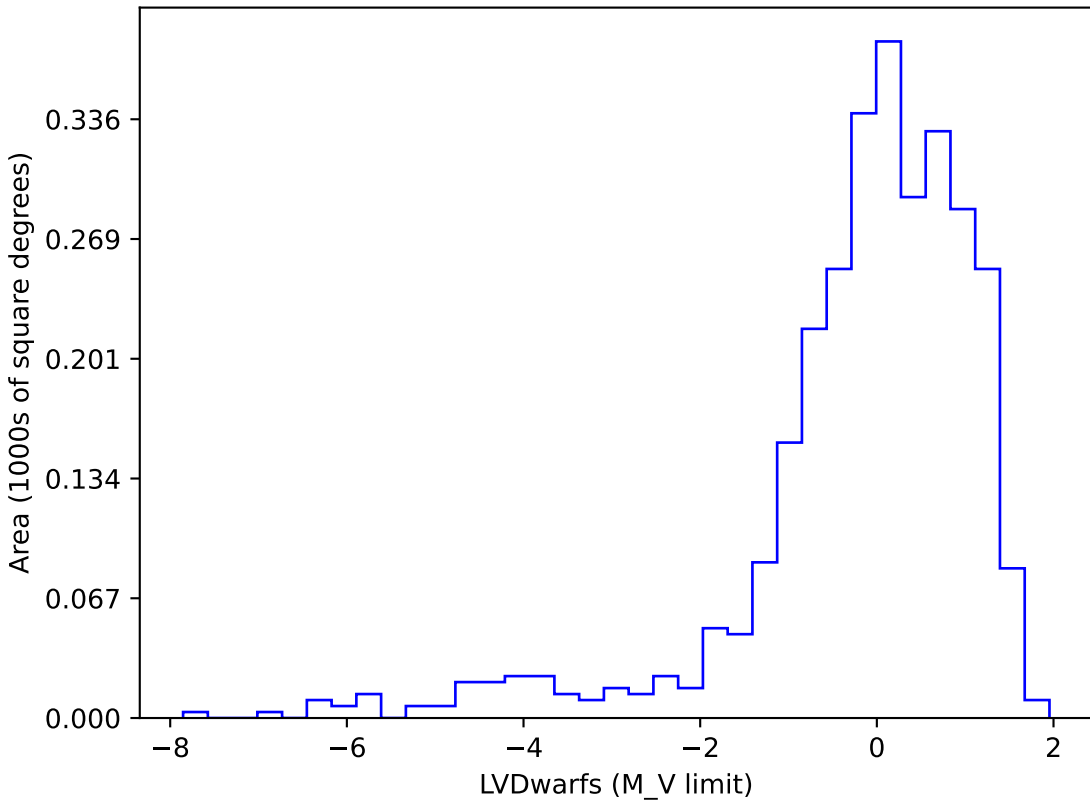
ddf_acor_sf10_lsf20_lsr10_v3.4_10yrs gi SCP: LVDwarfs
