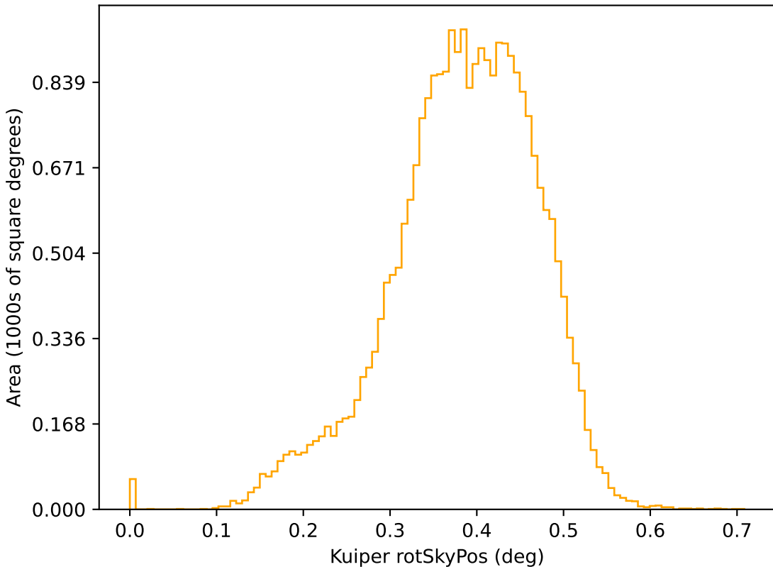
ddf_acor_sf10_lsf20_lsr10_v3.4_10yrs r: Kuiper rotSkyPos
