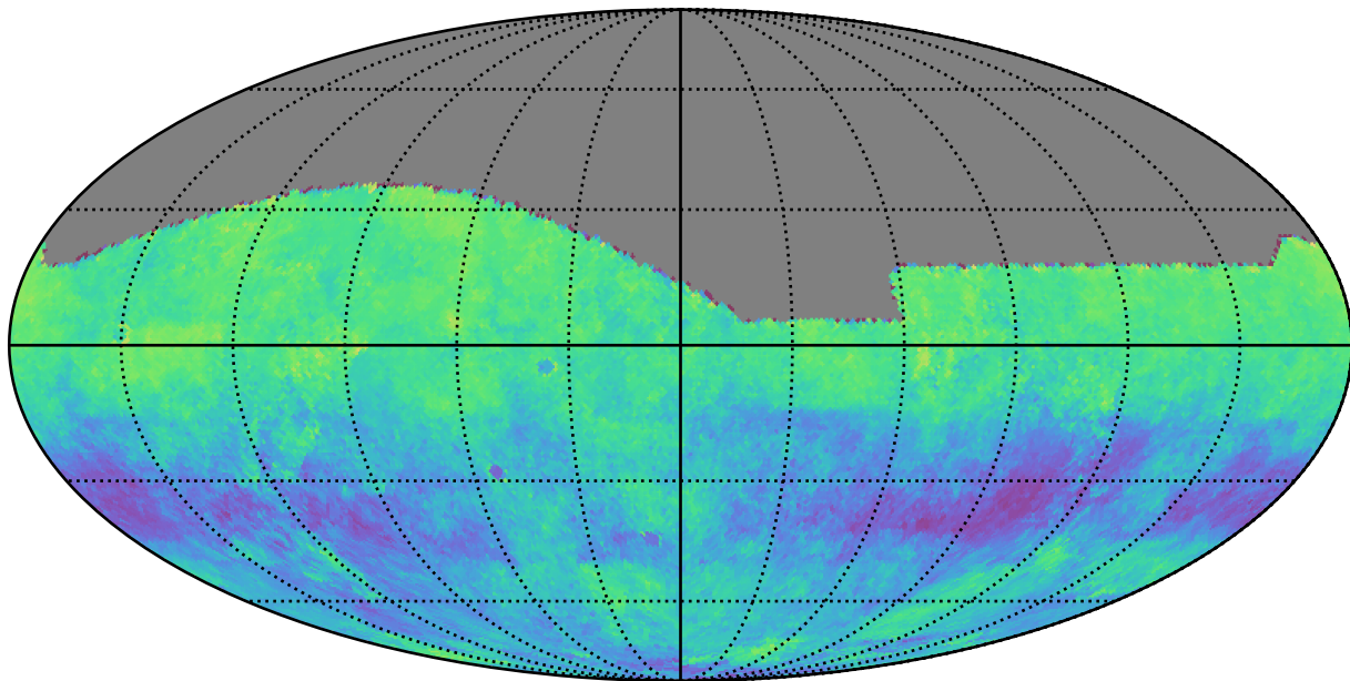
ddf_acor_sf10_lsf20_lsr10_v3.4_10yrs g: Kuiper rotSkyPos
