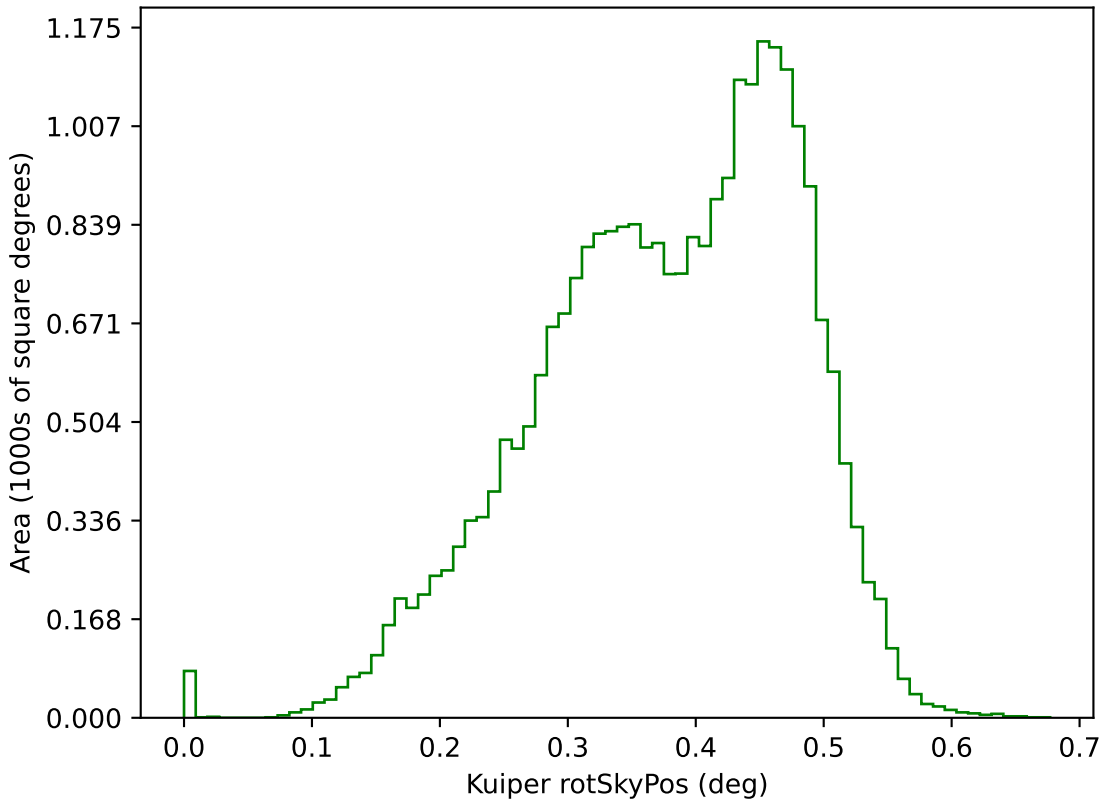
ddf_acor_sf10_ls20_lsr10_v3.4_10yrs g: Kuiper rotSkyPos
