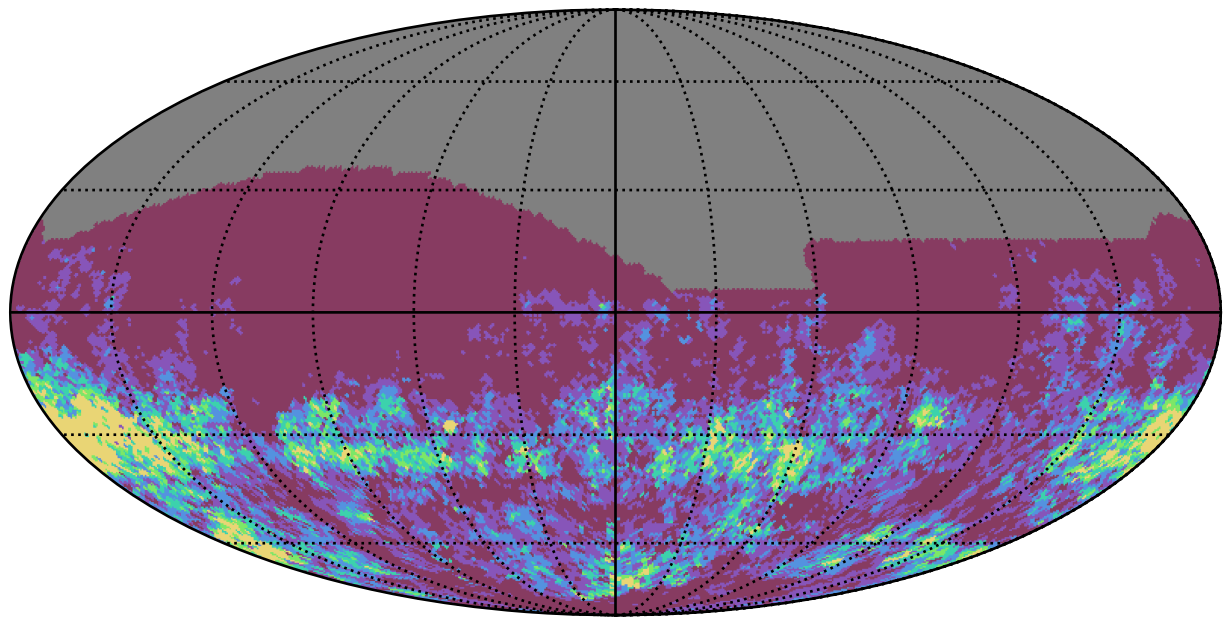
ddf_acor_sf10_lsf20_lsr10_v3.4_10yrs r band: Gaps_7hr
