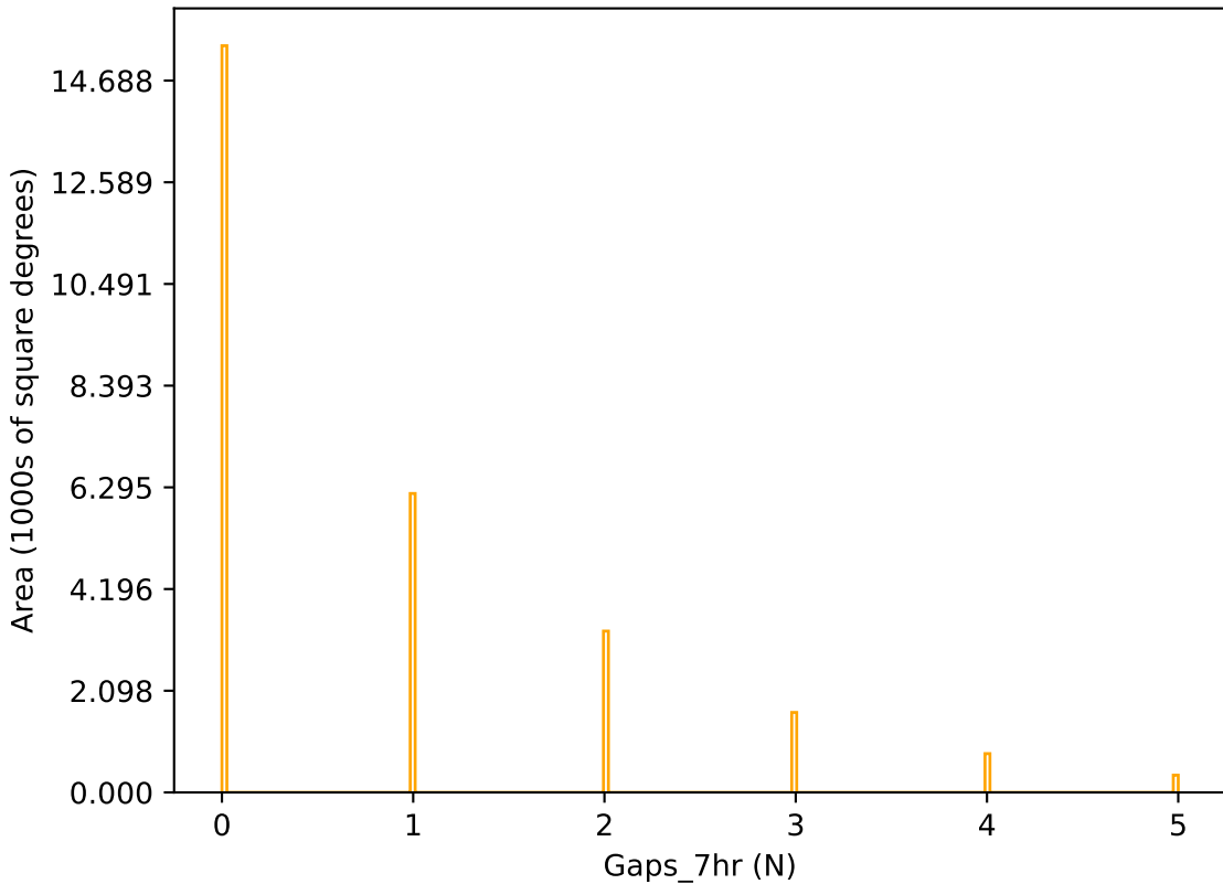
ddf_acor_sf10_lsf20_lsr10_v3.4_10yrs r band: Gaps_7hr
