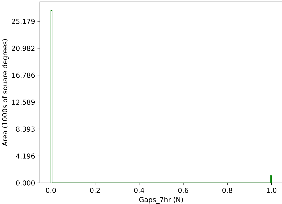
ddf_acor_sf10_lsf20_lsr10_v3.4_10yrs g band: Gaps_7hr
