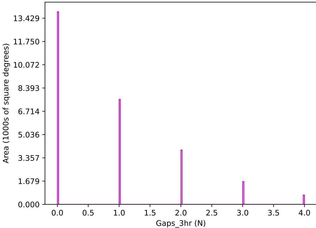
ddf_acor_sf10_lsf20_lsr10_v3.4_10yrs z band: Gaps_3hr
