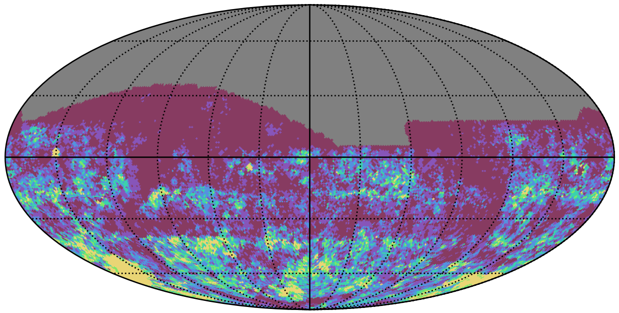
ddf_acor_sf10_lsf20_lsr10_v3.4_10yrs r band: Gaps_3hr
