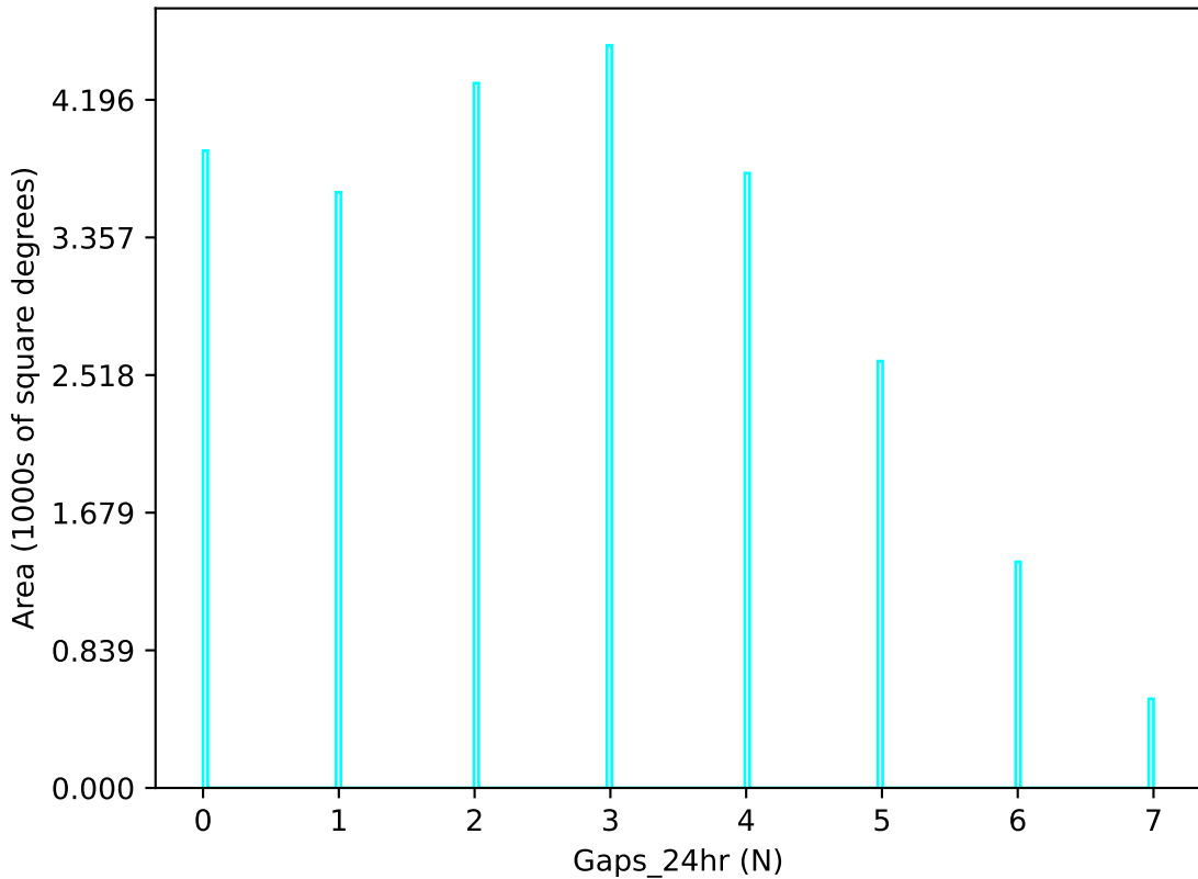
ddf_acor_sf10_lsf20_lsr10_v3.4_10yrs u band: Gaps_24hr
