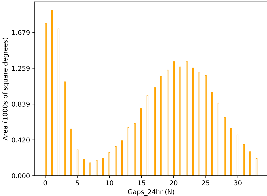
ddf_acor_sf10_lsf20_lsr10_v3.4_10yrs r band: Gaps_24hr
