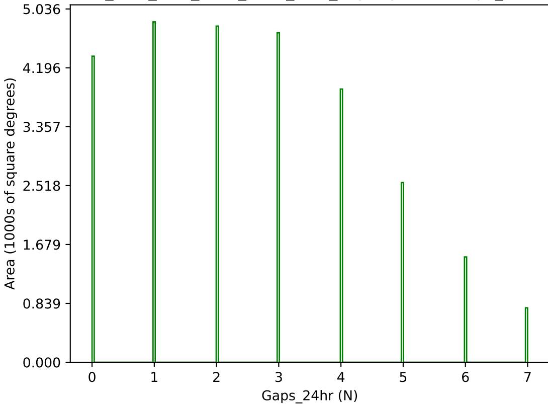
ddf_acor_sf10_lsf20_lsr10_v3.4_10yrs g band: Gaps_24hr
