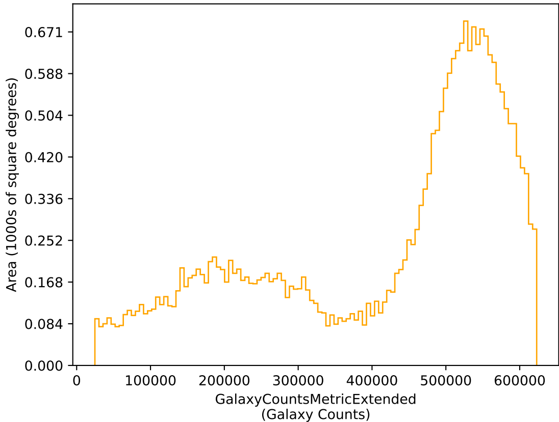
ddf_acor_sf10_lsf20_lsr10_v3.4_10yrs r: GalaxyCountsMetricExtended
