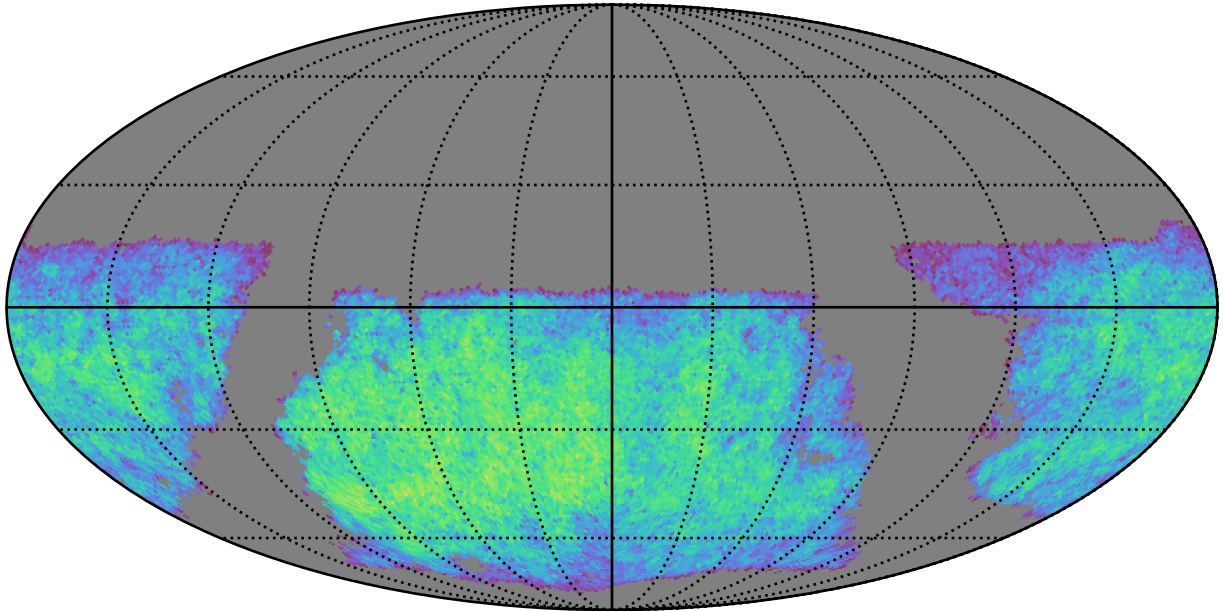
ddf_acor_sf10_lsf20_lsr10_v3.4_10yrs i band non-DD year 1: ExgalM5WithCuts
