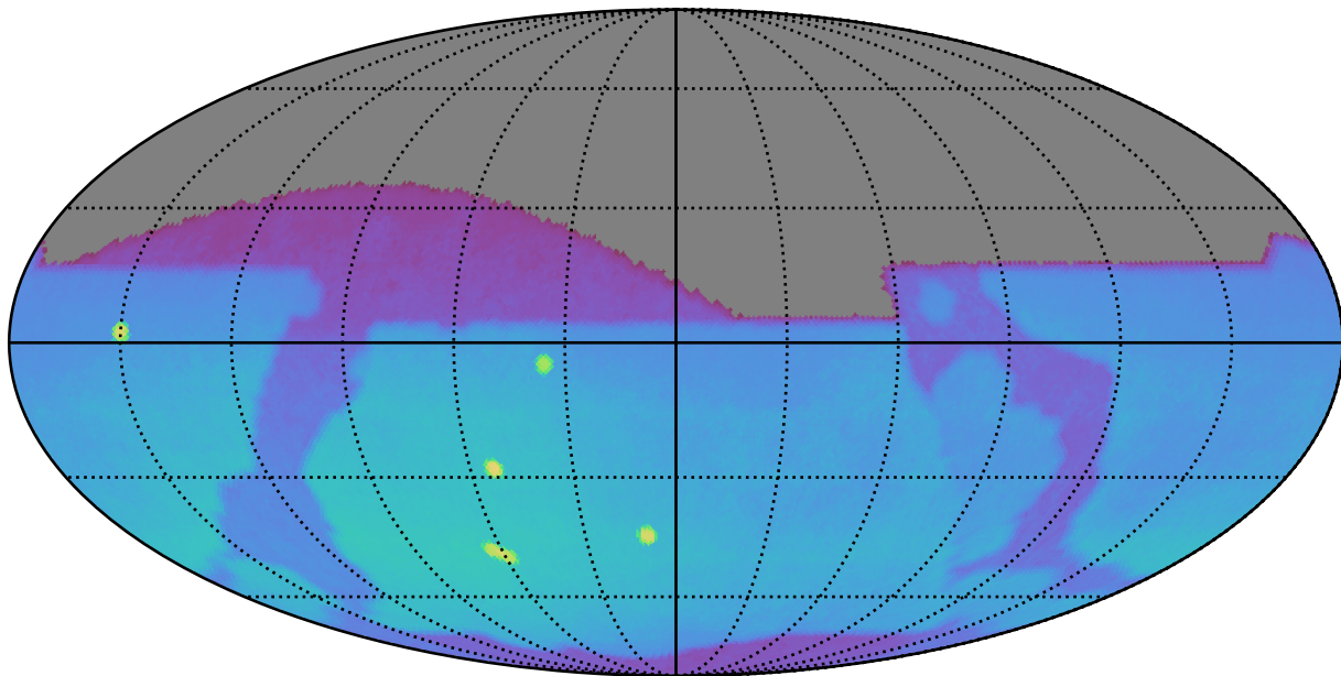
ddf_acor_sf10_lsf20_lsr10_v3.4_10yrs : Brown Dwarf, L7
