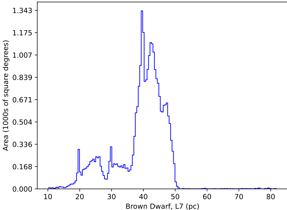
ddf_acor_sf10_lsf20_lsr10_v3.4_10yrs : Brown Dwarf, L7
