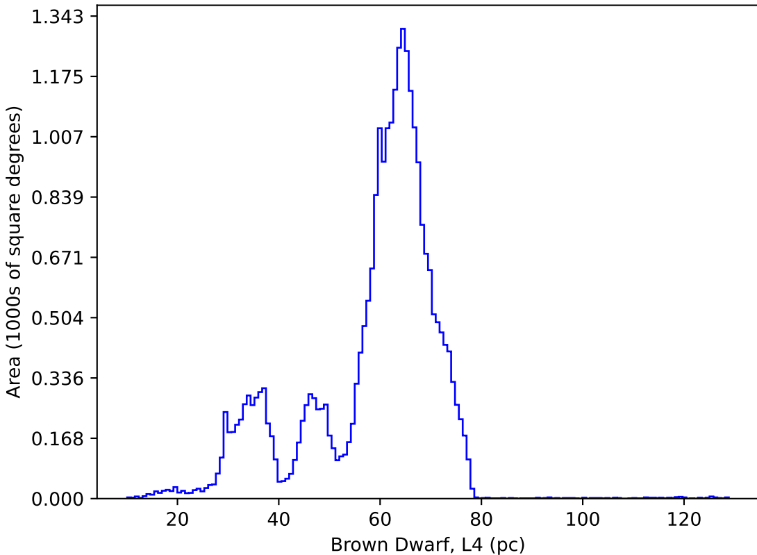
ddf_acor_sf10_lsf20_lsr10_v3.4_10yrs : Brown Dwarf, L4
