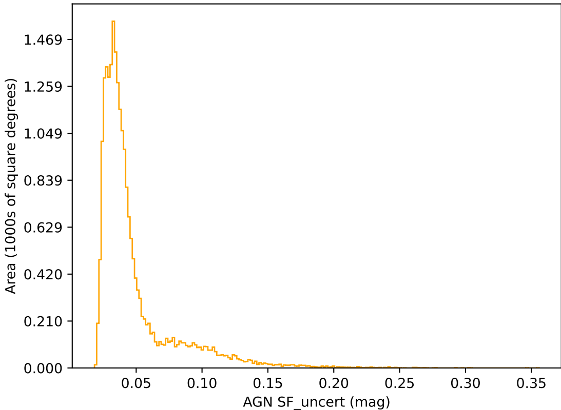
ddf_acor_sf10_lsf20_lsr10_v3.4_10yrs r band: AGN SF_uncert
