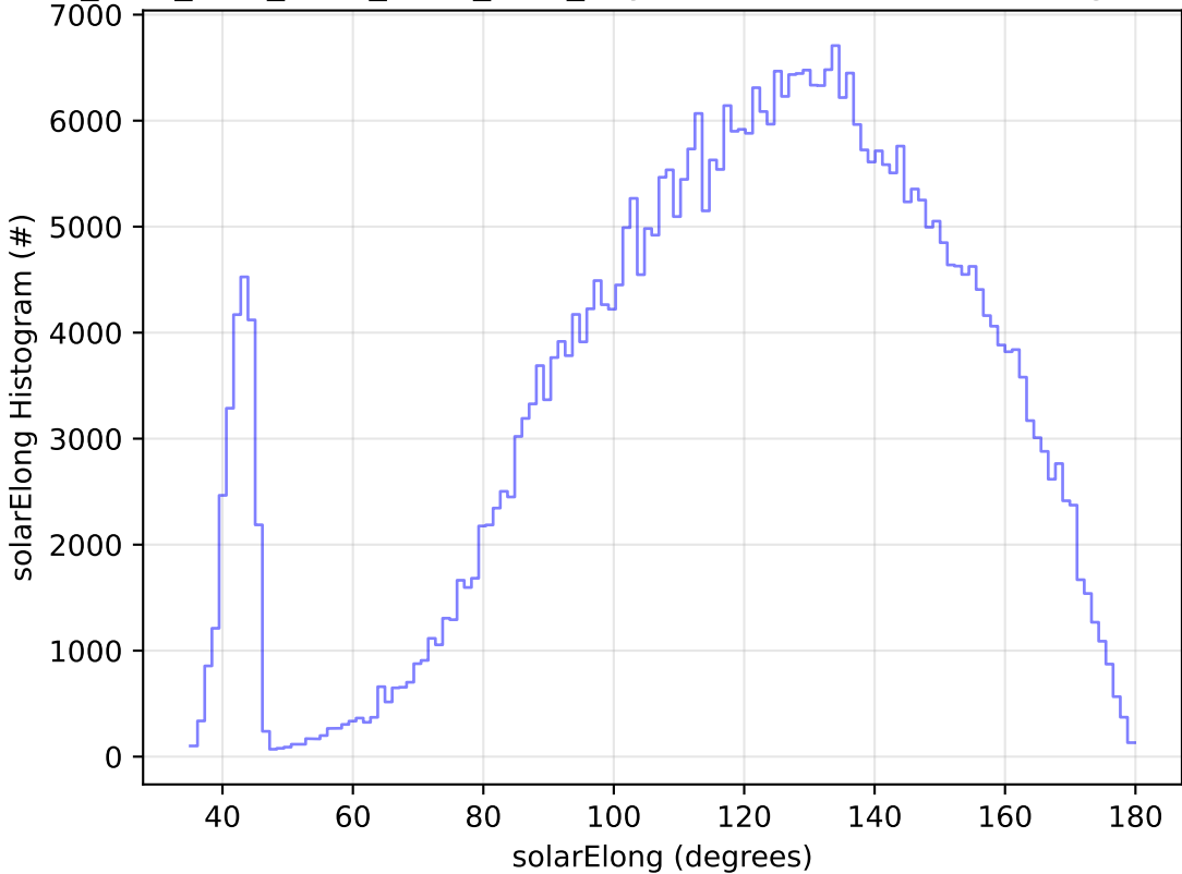
ddf_acor_sf10_lsf20_lsr10_v3.4_10yrs WFD z band: solarElong Histogram
