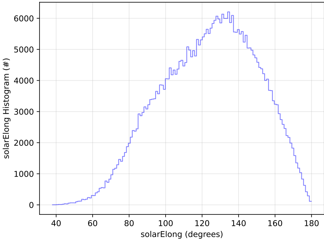
ddf_acor_sf10_lsf20_lsr10_v3.4_10yrs WFD y band: solarElong Histogram
