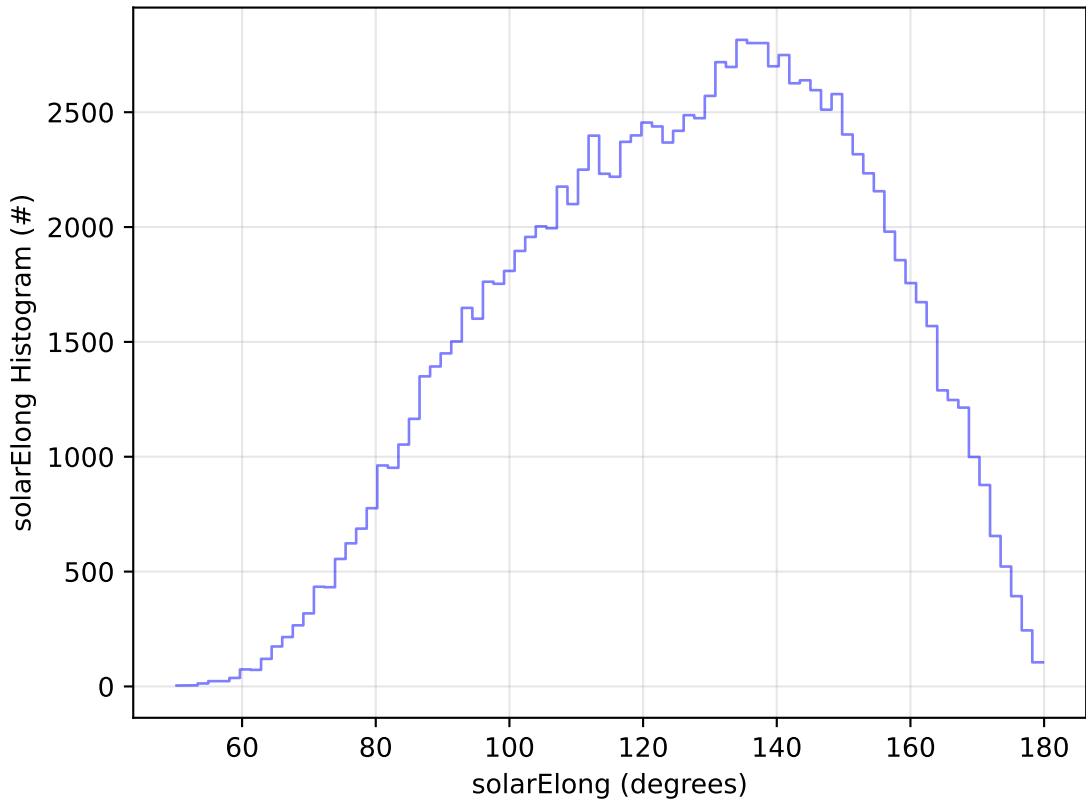
ddf_acor_sf10_lsf20_lsr10_v3.4_10yrs WFD u band: solarElong Histogram
