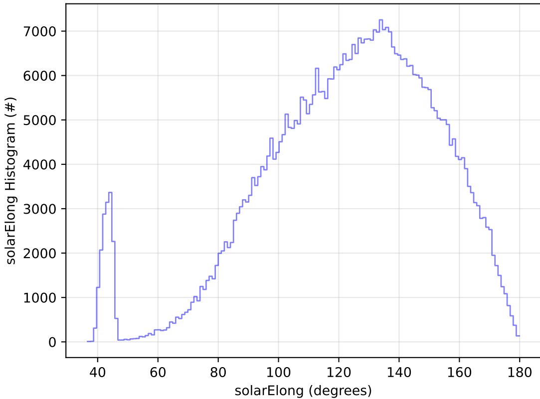
ddf_acor_sf10_lsf20_lsr10_v3.4_10yrs WFD r band: solarElong Histogram
