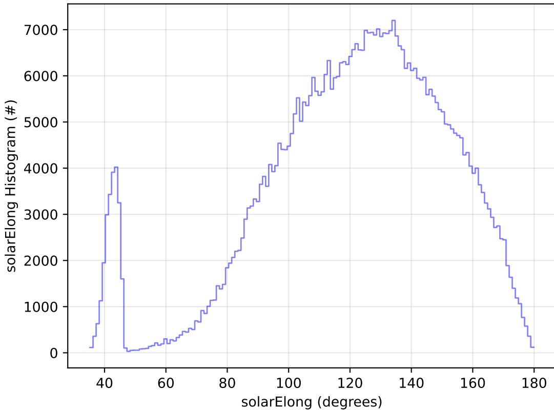
ddf_acor_sf10_lsf20_lsr10_v3.4_10yrs WFD i band: solarElong Histogram
