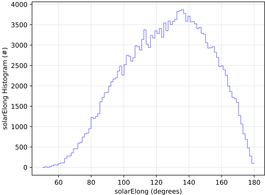
ddf_acor_sf10_lsf20_lsr10_v3.4_10yrs WFD g band: solarElong Histogram
