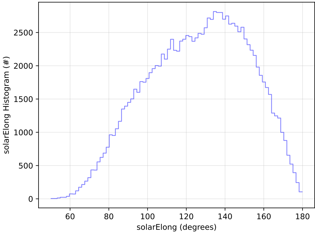
ddf_acor_sf10_lsf20_lsr10_v3.4_10yrs All sky u band: solarElong Histogram
