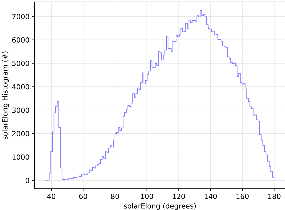
ddf_acor_sf10_lsf20_lsr10_v3.4_10yrs All sky r band: solarElong Histogram
