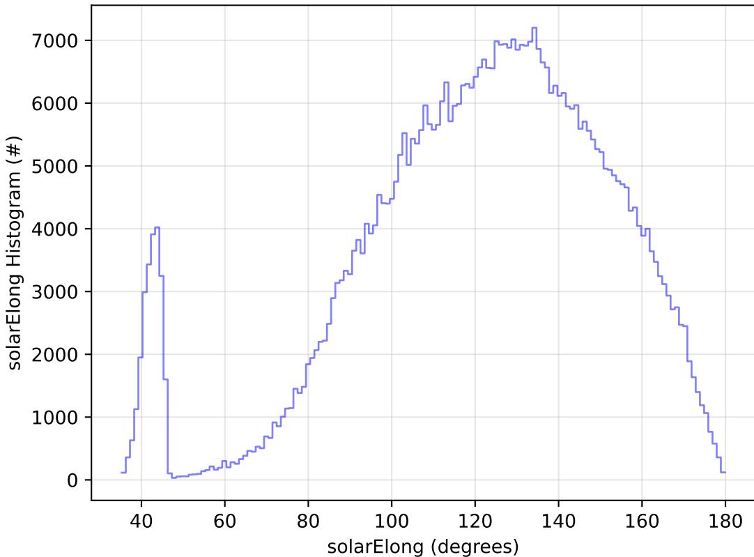
ddf_acor_sf10_lsf20_lsr10_v3.4_10yrs All sky i band: solarElong Histogram
