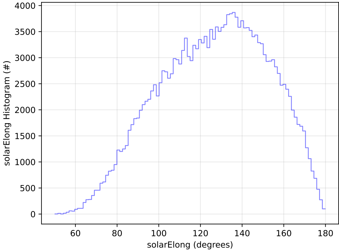
ddf_acor_sf10_lsf20_lsr10_v3.4_10yrs All sky g band: solarElong Histogram
