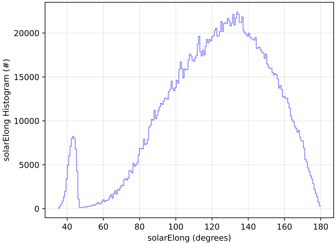
ddf_acor_sf10_lsf20_lsr10_v3.4_10yrs All sky all bands: solarElong Histogram
