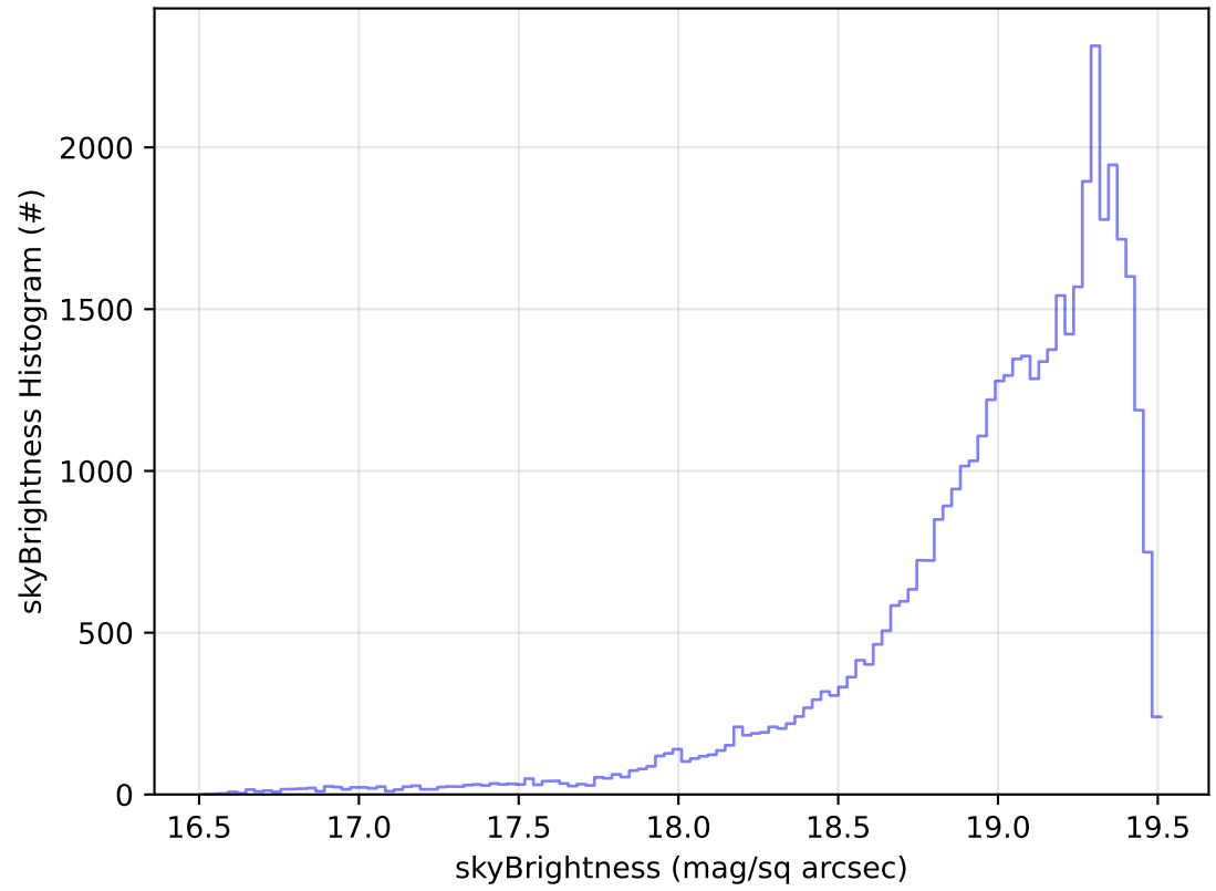
ddf_acor_sf10_lsf20_lsr10_v3.4_10yrs Yr 1 z band: skyBrightness Histogram
