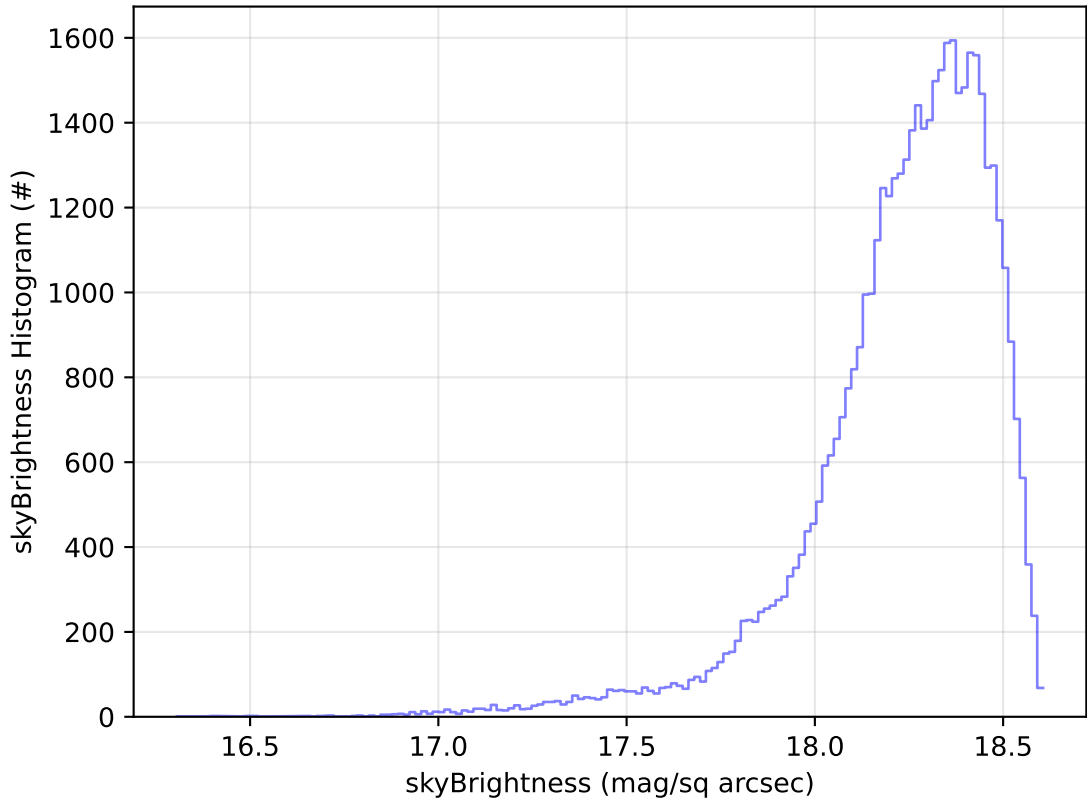
ddf_acor_sf10_lsf20_lsr10_v3.4_10yrs Yr 1 y band: skyBrightness Histogram
