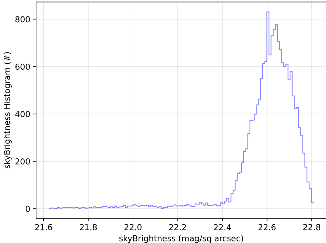
ddf_acor_sf10_lsf20_lsr10_v3.4_10yrs Yr 1 u band: skyBrightness Histogram
