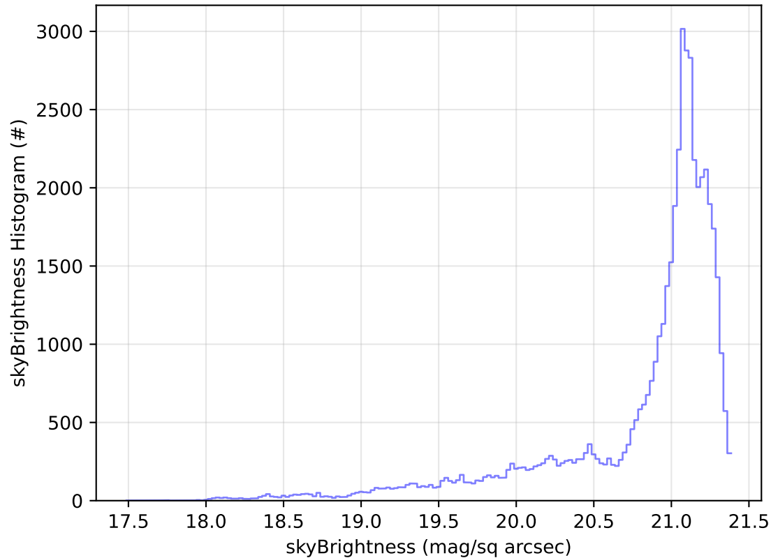
ddf_acor_sf10_lsf20_lsr10_v3.4_10yrs Yr 1 r band: skyBrightness Histogram
