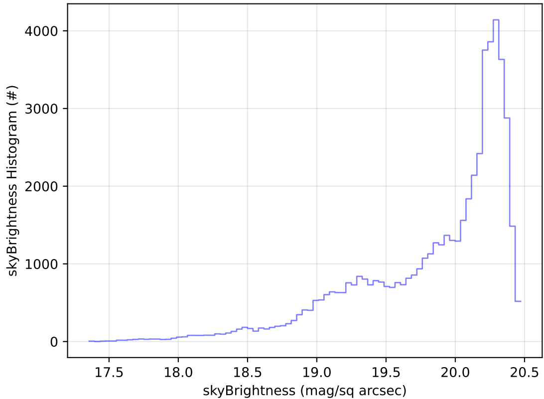
ddf_acor_sf10_lsf20_lsr10_v3.4_10yrs Yr 1 i band: skyBrightness Histogram
