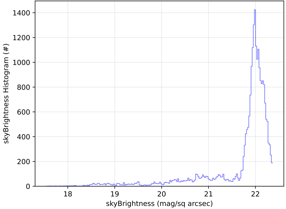
ddf_acor_sf10_lsf20_lsr10_v3.4_10yrs Yr 1 g band: skyBrightness Histogram
