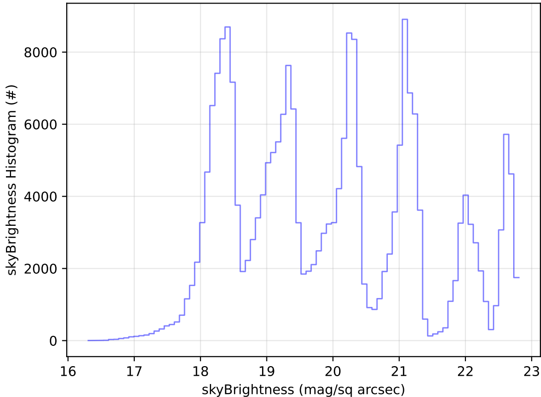
ddf_acor_sf10_lsf20_lsr10_v3.4_10yrs Yr 1 all bands: skyBrightness Histogram
