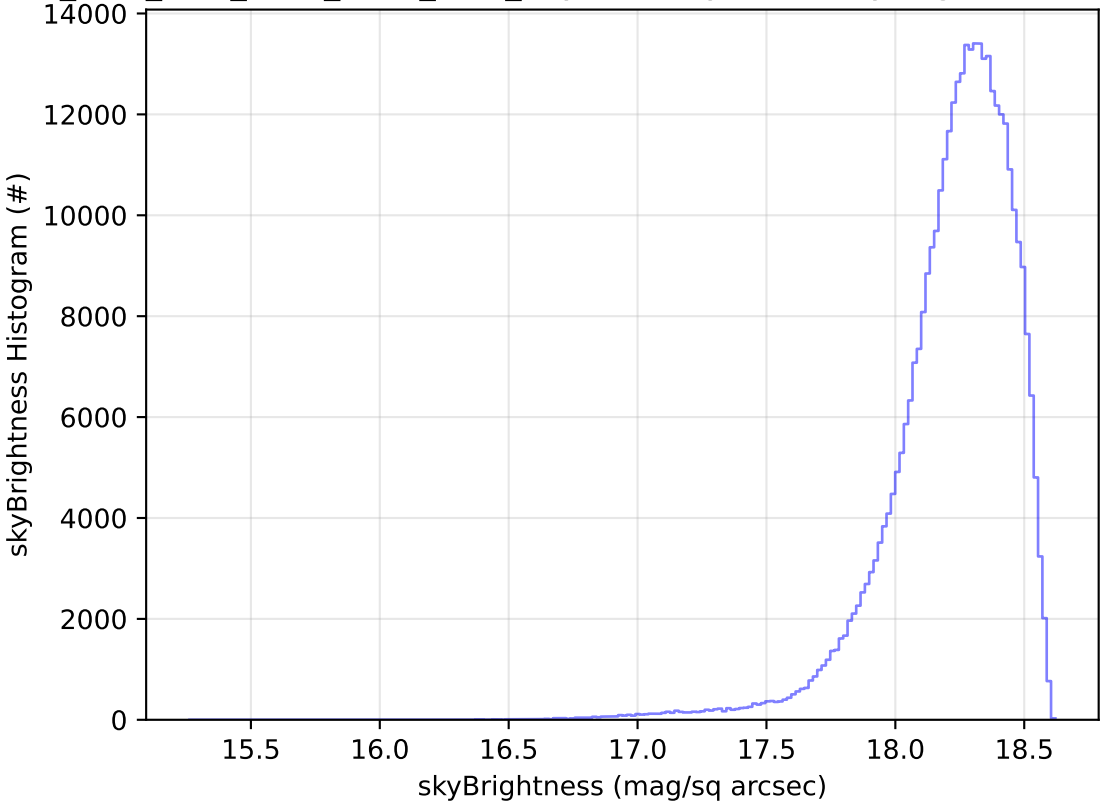
ddf_acor_sf10_lsf20_lsr10_v3.4_10yrs WFD y band: skyBrightness Histogram
