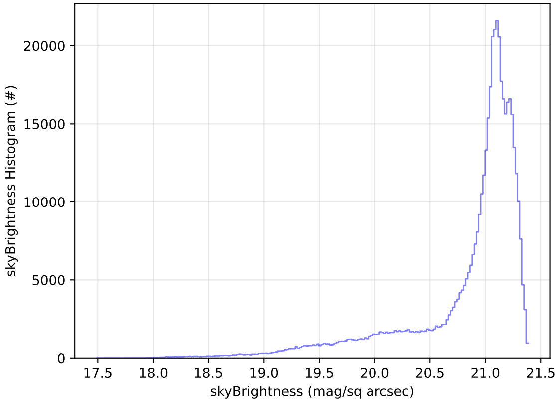
ddf_acor_sf10_lsf20_lsr10_v3.4_10yrs WFD r band: skyBrightness Histogram
